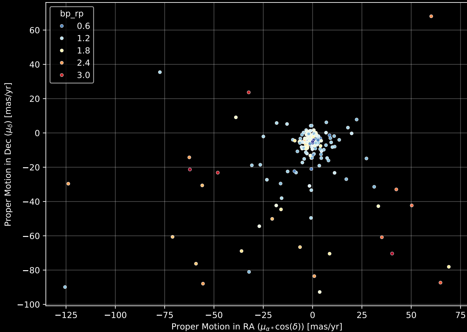
APOGEE DR17 Field: [K2_C7_012-13_btx] Proper Motion Diagram (n= 183)
