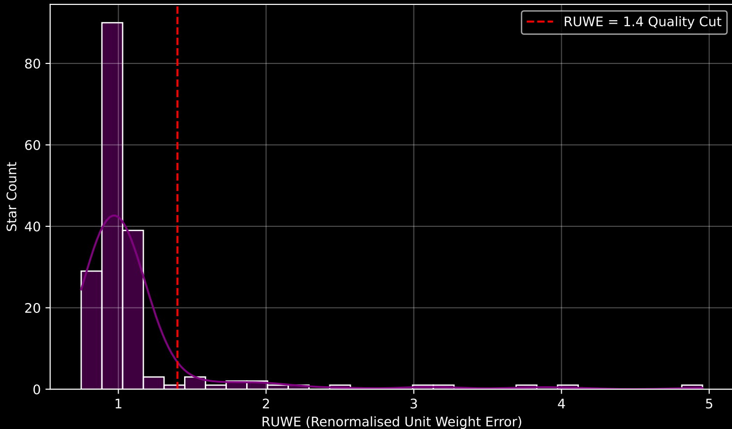
GAPOGEE DR17 Field [K2_C7_012-13_btx] RUWE Distribution (n= 178)
