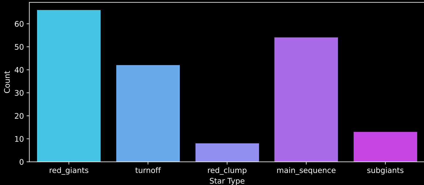
APOGEE DR17 Field: [K2_C7_012-13_btx] Count plot of Star Type
