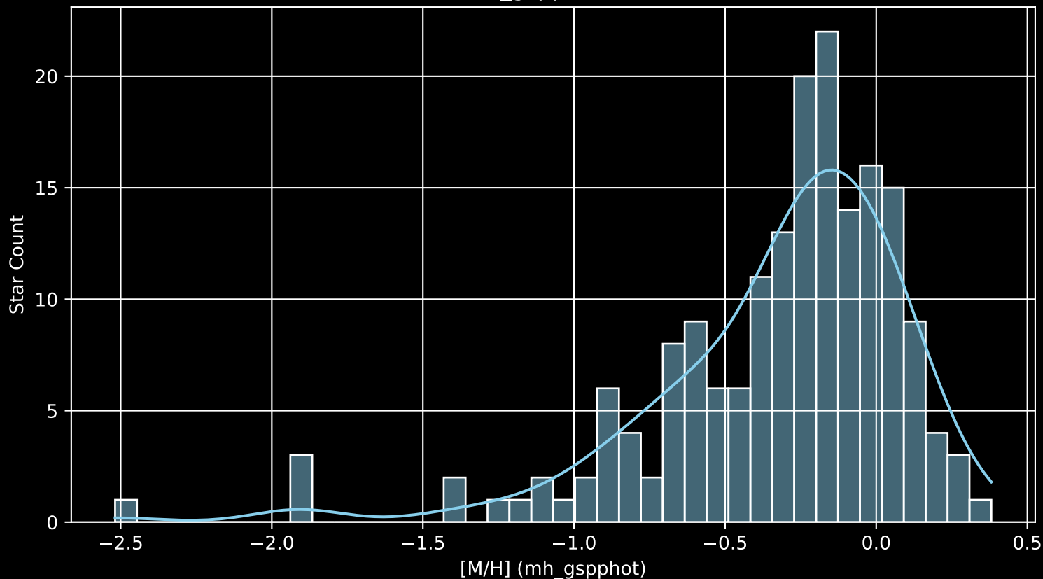
APOGEE DR17 Field: [K2_C7_012-13_btx [M/H] (mh_gspphot) (n= 182)
