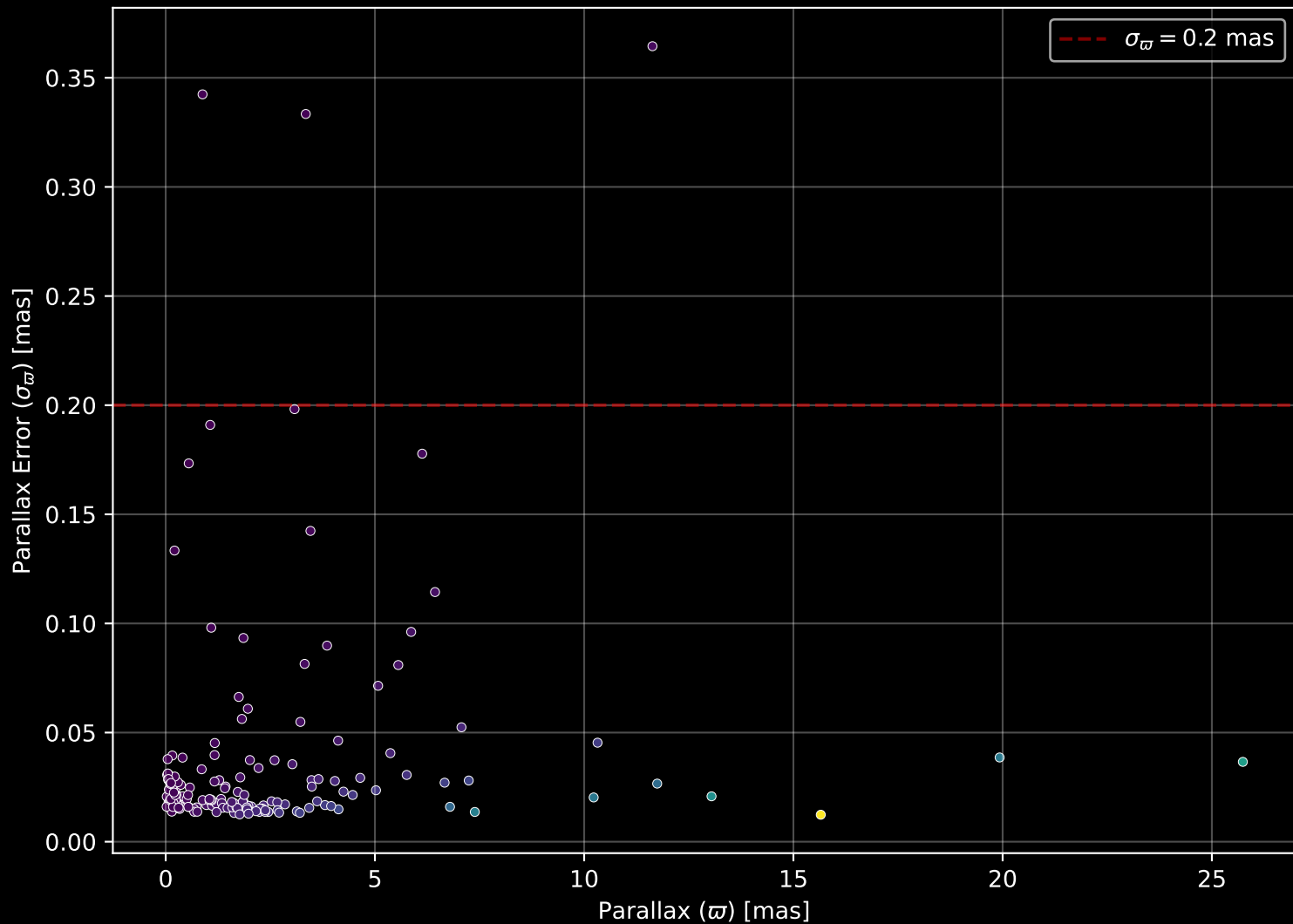
APOGEE DR17 Field: [K2_C7_012-13_btx] Parallax Quality (n= 183)
